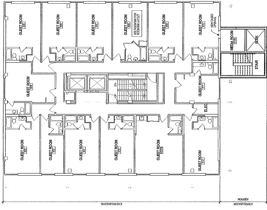
1 FOURTH FLOOR PLAN (5 & 6TH FLOOR SIMILAR) 1/8" = 1'-0"
