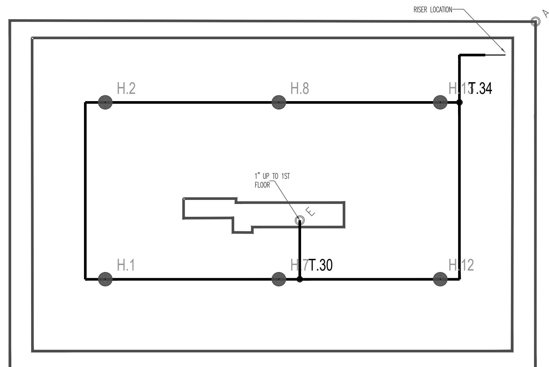
FIRE SPRINKLER PLAN - BASEMENT 1/4" = 1'-0" FLOOR EL. (90'-0")
