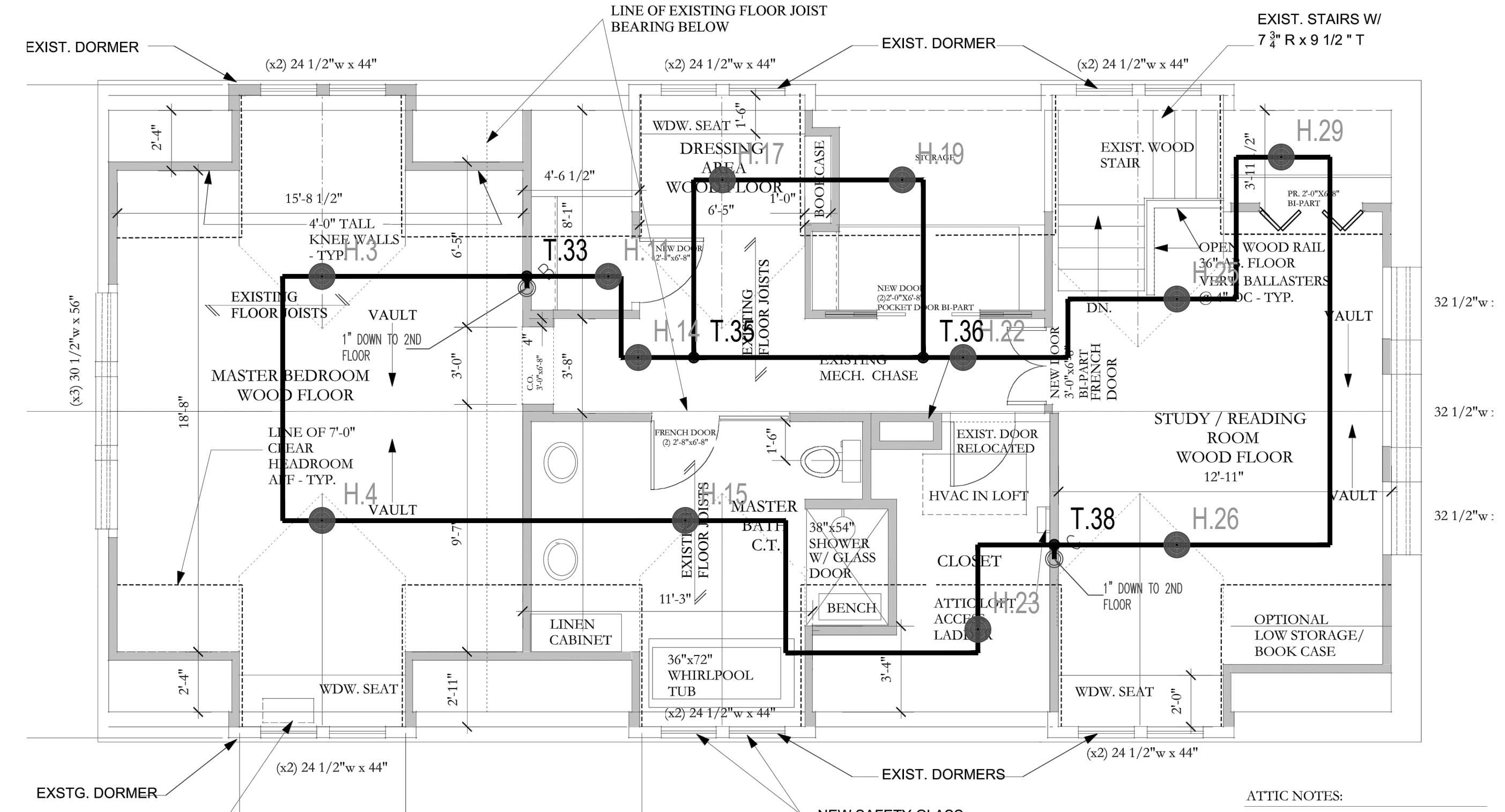
FIRE SPRINKLER PLAN - 3RD FLOOR 1/4" = 1'-0" FLOOR EL. (120'-0")
