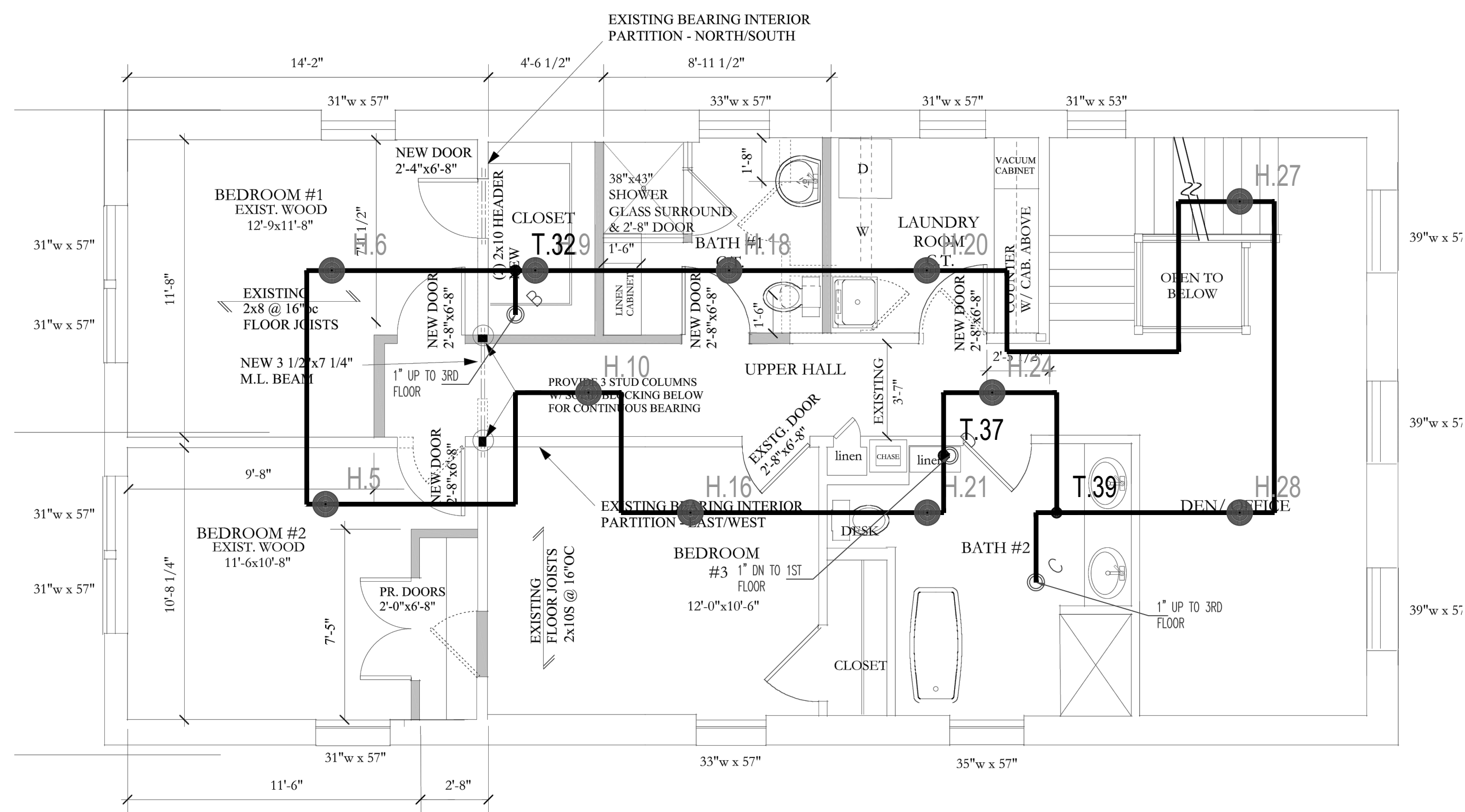
FIRE SPRINKLER PLAN - 2ND FLOOR 1/4" = 1'-0" FLOOR EL. (110'-0")
