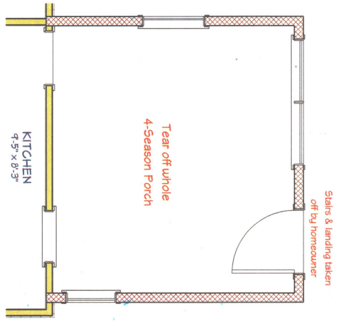
DEMO PLAN - 4-SEASON PORCH Scale: 1/4" = 1' - 0"
