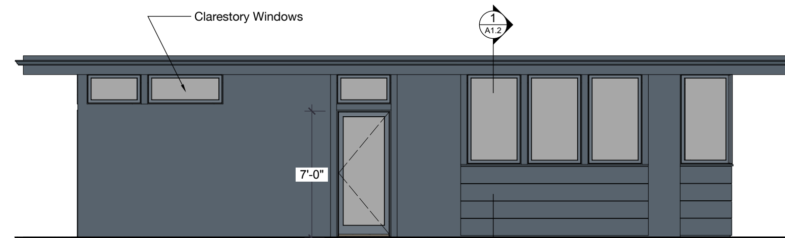
3 East Elevation Scale 1/4" : 1' (11"x17")
