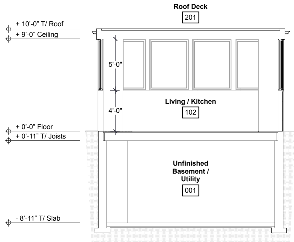
1 Section Scale 1/4" : 1' (11"x17")
