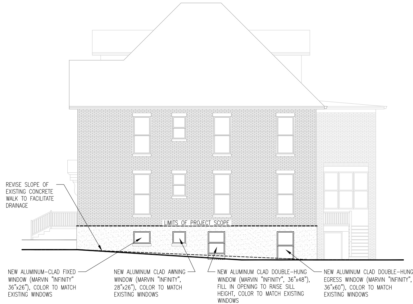
2 WEST ELEVATION - PROPOSED SCALE: 3/32"=1'-0"
