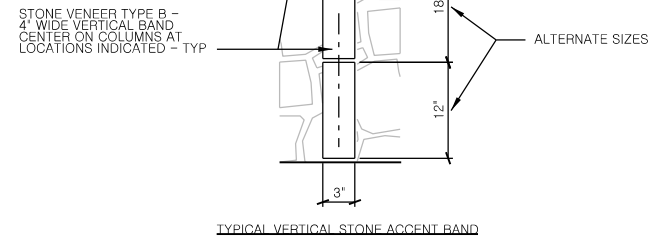
TYPICAL VERTICAL STONE ACCENT BAND
