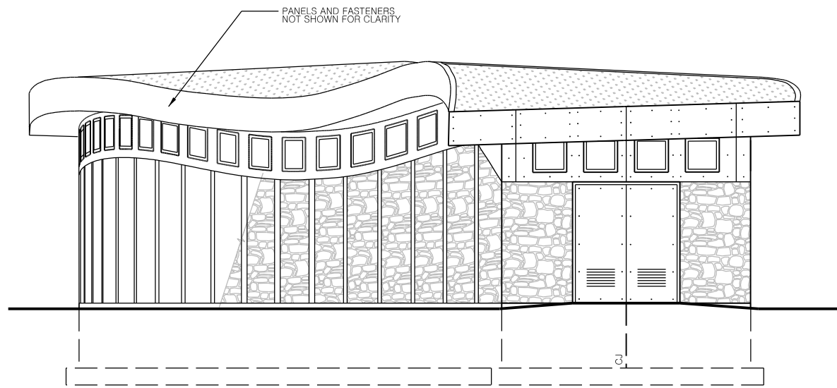
SOUTH ELEVATION
