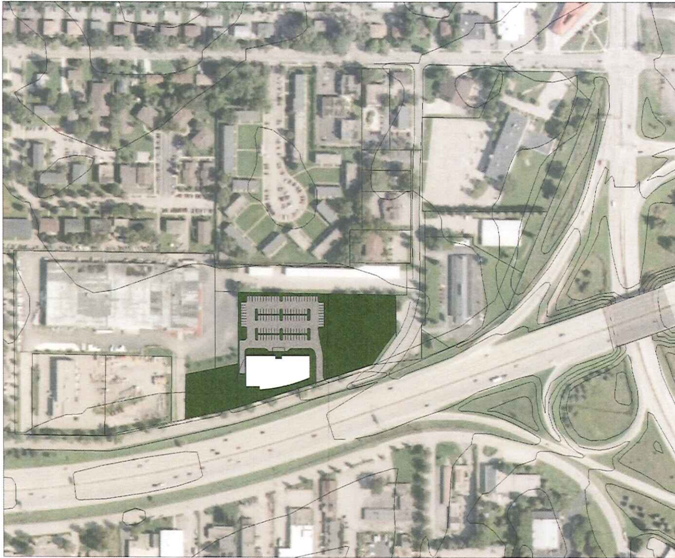
Aerial Sketch - Phase One Ann Street Conceptual Site Design 11.05.10
