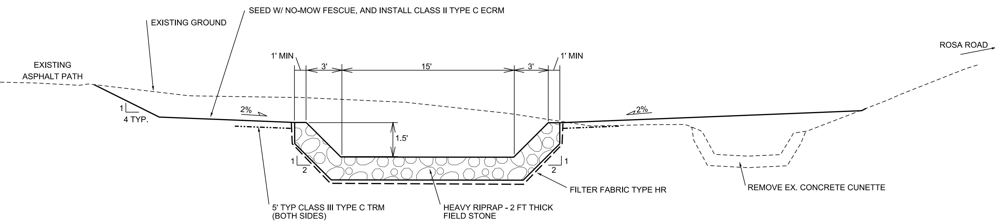
TYPICAL SECTION STONE CHANNEL - NOT TO SCALE
