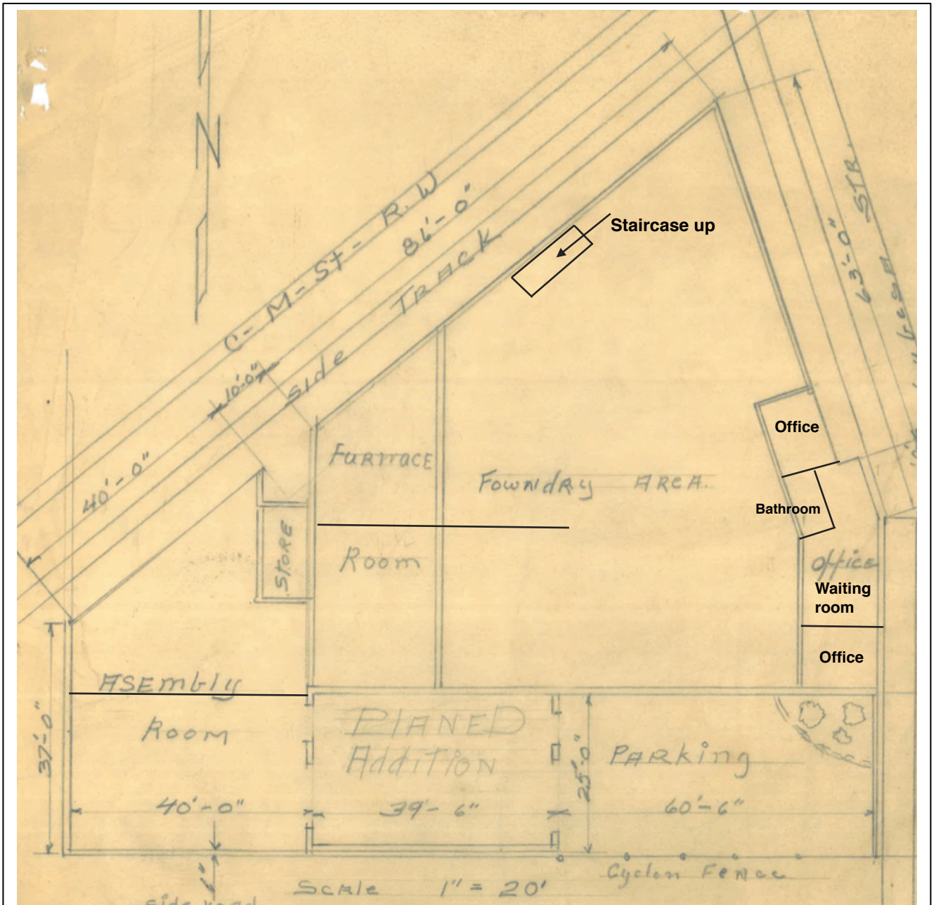
Figure 7. Madison Brass Works Madison, Dane County, Wisconsin Floor Plan
