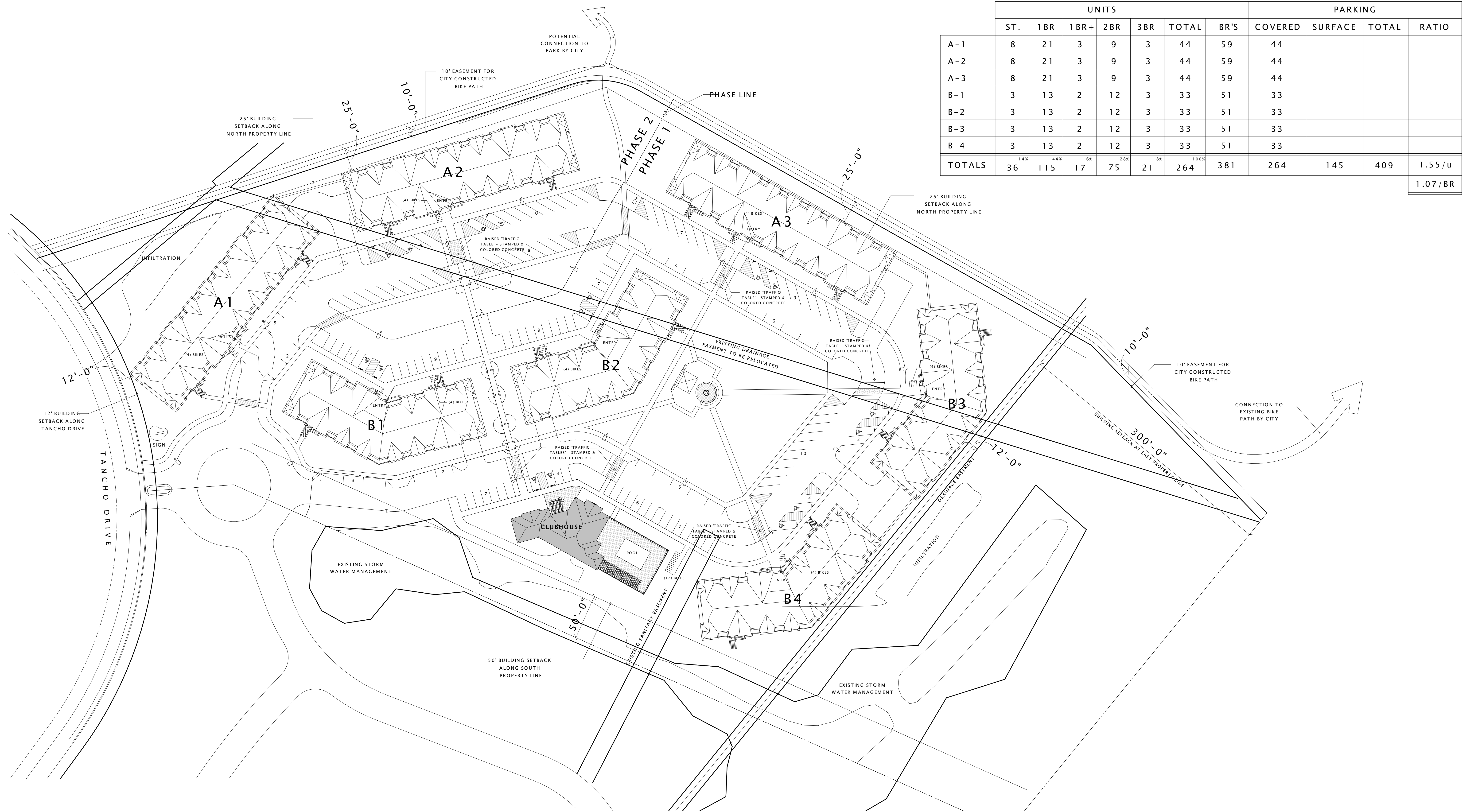
16 ARCHITECTURAL SITE PLAN - OVERALL 1" = 50'-0"
