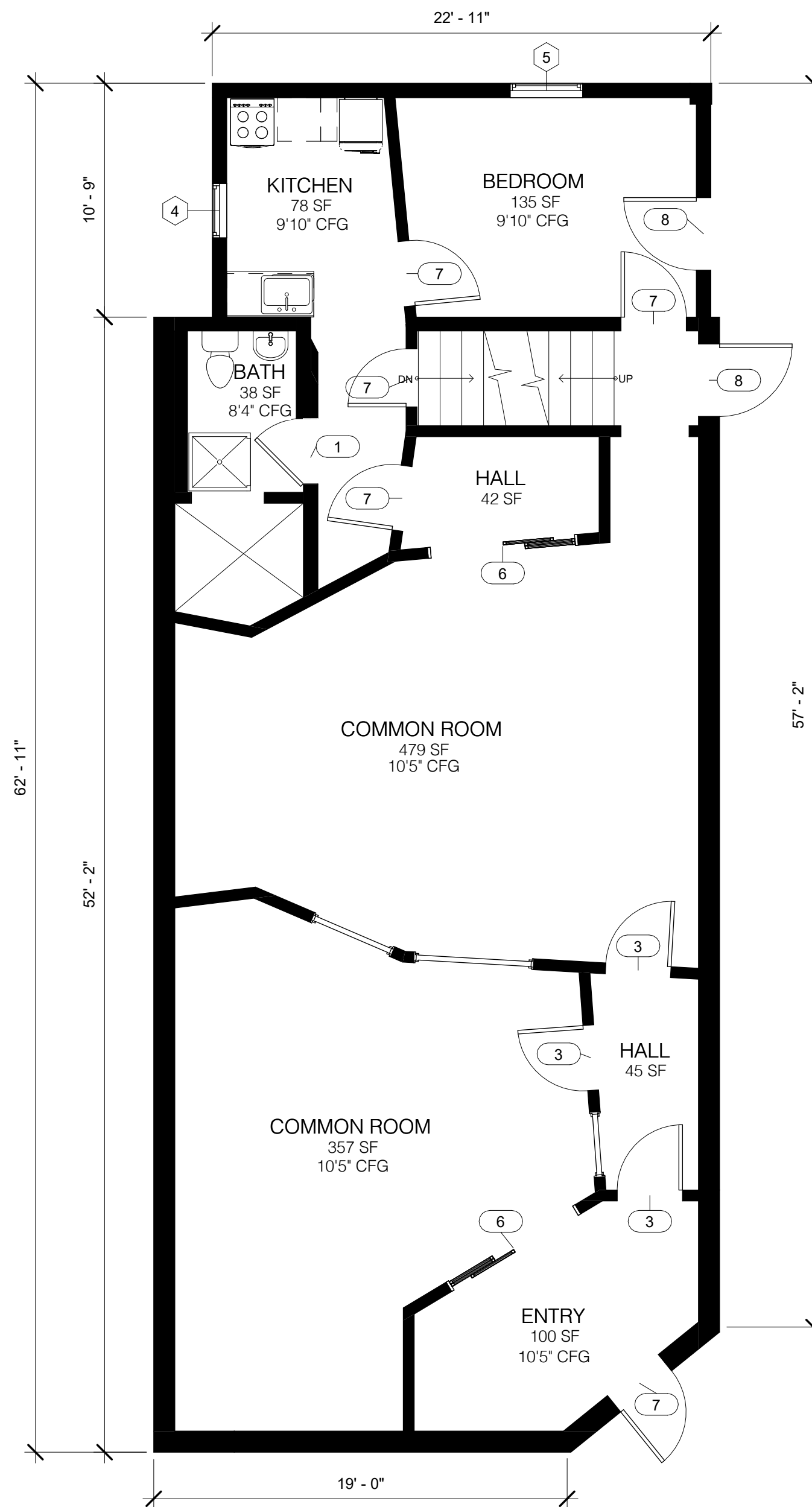
2 1st FLOOR PLAN
