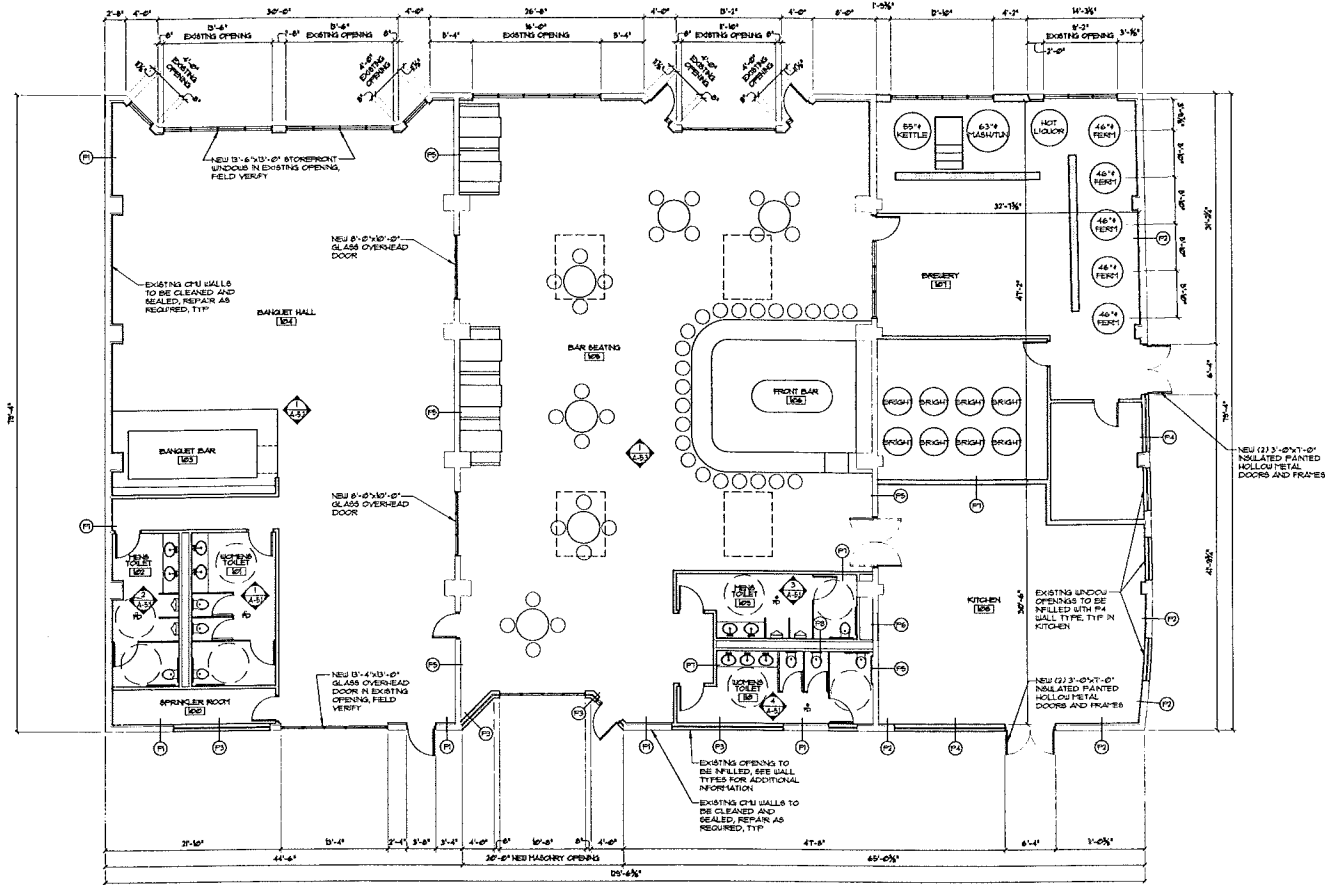
1 PROPOSED BREW PUB LAYOUT A-1.1 SCALE: 1/8" = 1' - 0" NORTH
