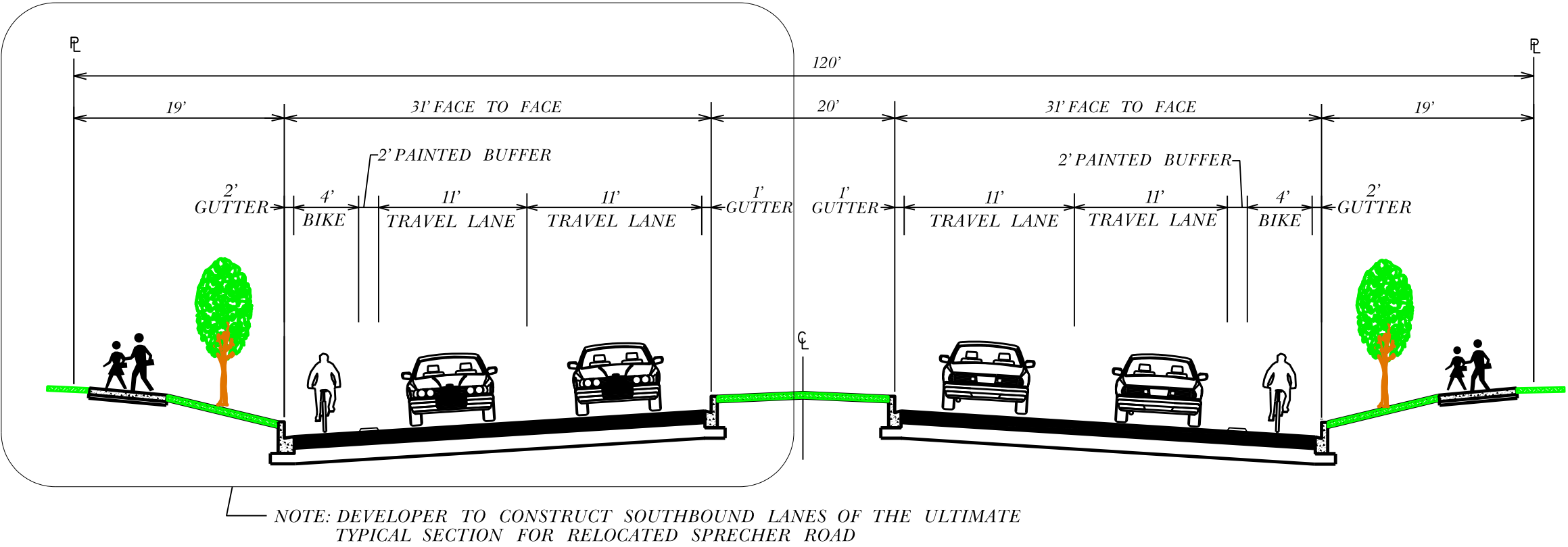
ULTIMATE TYPICAL FINISHED SECTION
