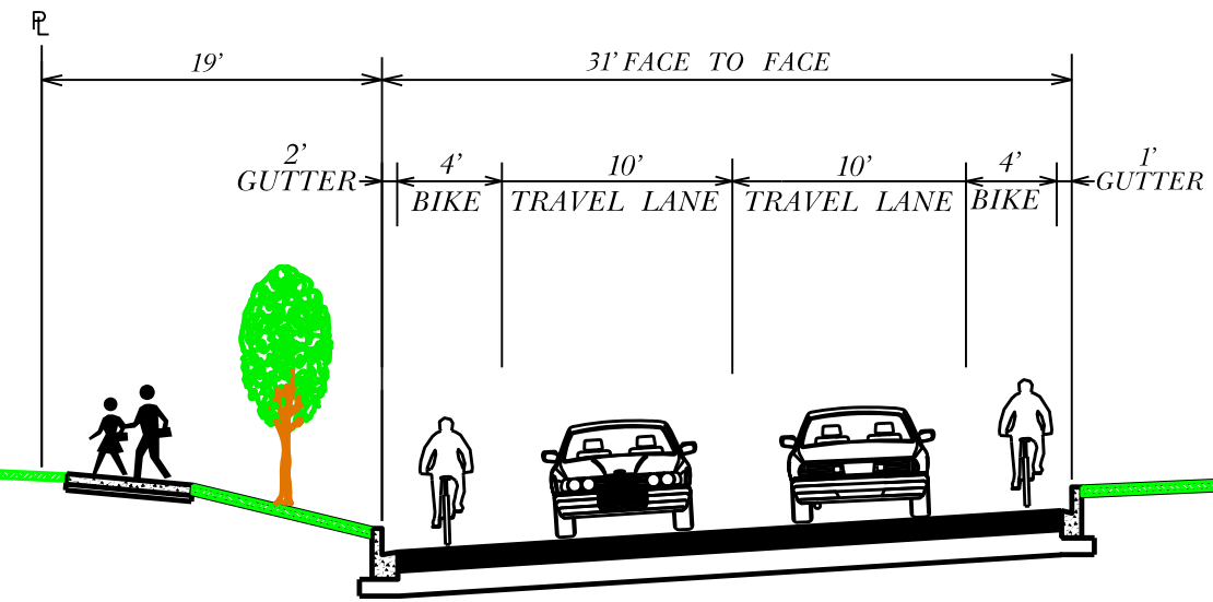
INTERIM TYPICAL SECTION – SPRECHER ROAD TO BE CONSTRUCTED BY DEVELOPER
