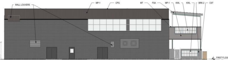
4 NORTH ELEVATION 332' x 1'-0"
