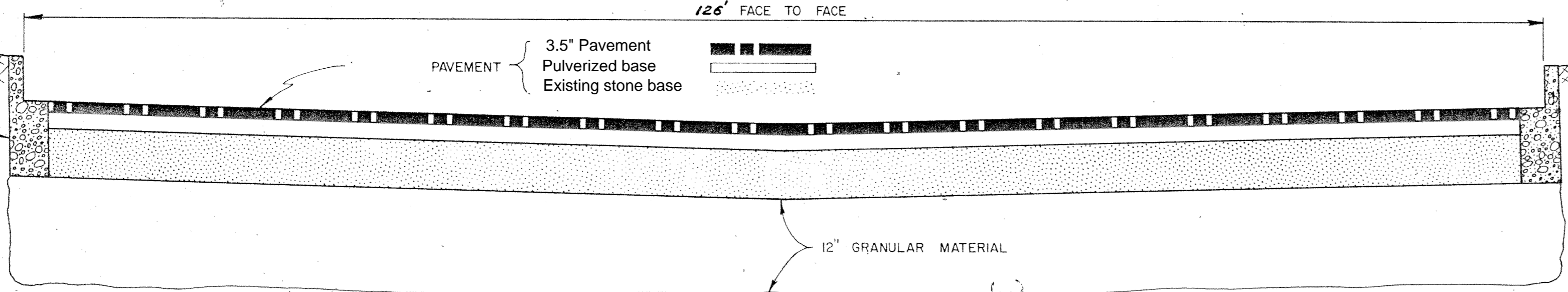
TYPICAL SECTION
