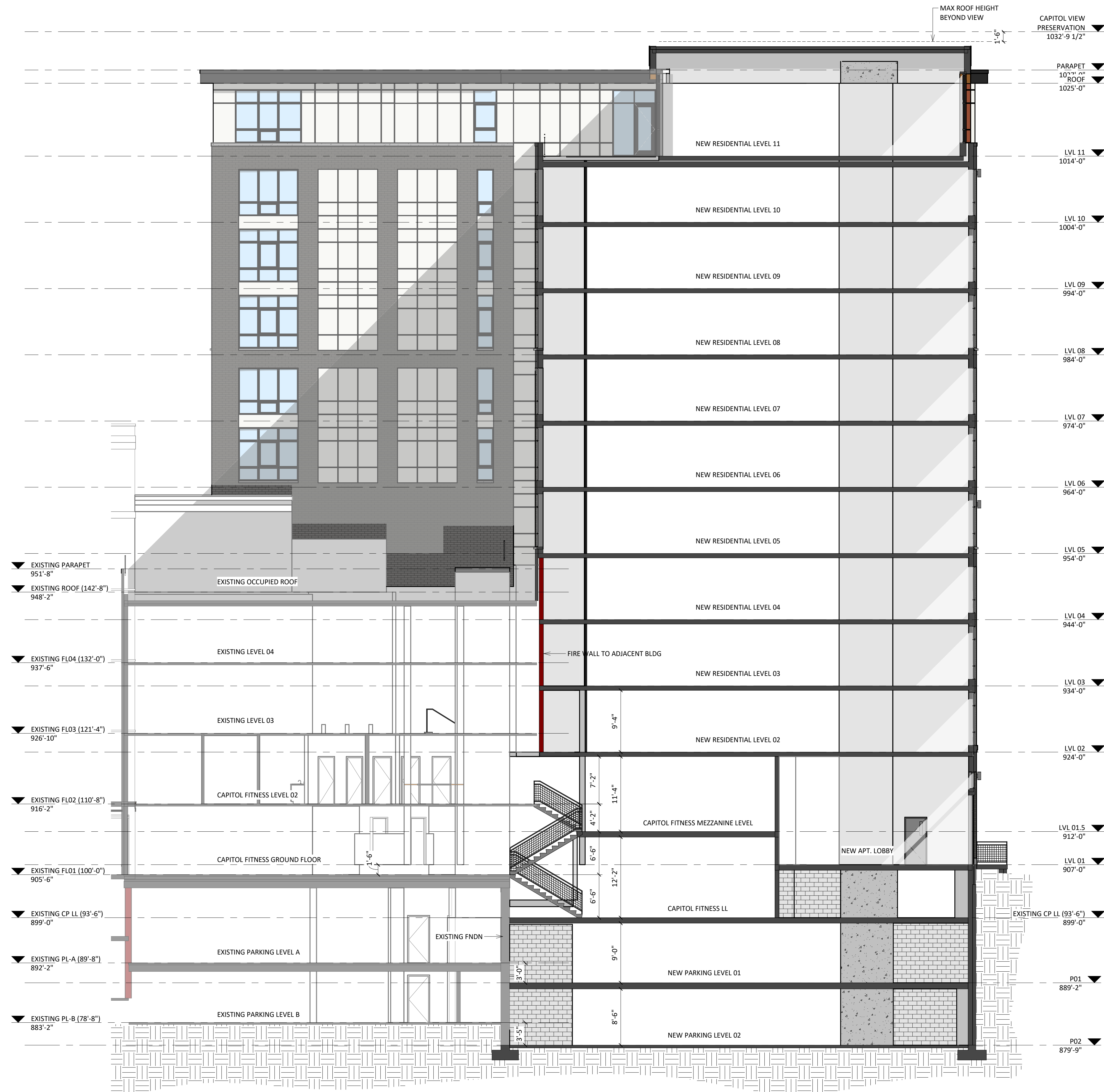
1 BUILDING SECTION 1/8" = 1'-0"
