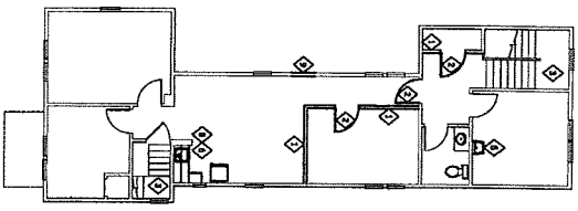
2 DEMO WORK SECOND FLOOR PLAN SCALE: 1/8" = 1'-0"
