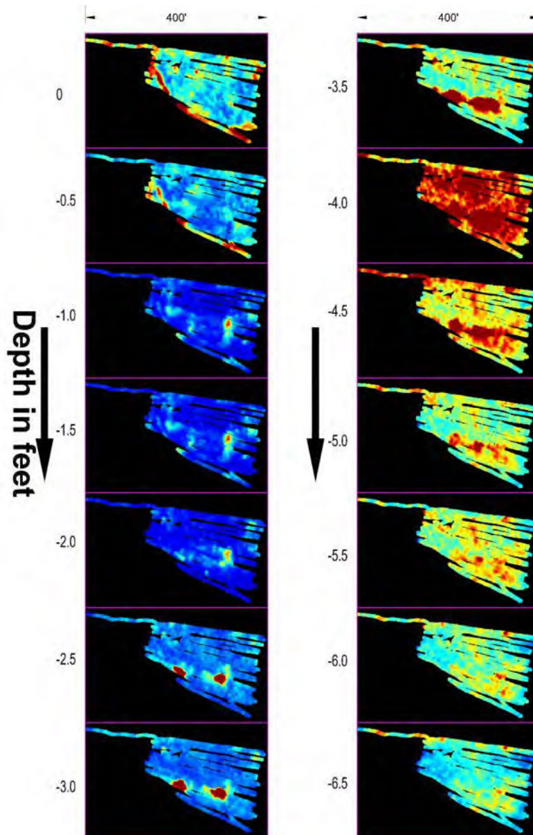
Figure 9: Horizontal slices at \frac{1}{2} foot increments showing multiple objects especially at depths 3.5 to 4.5.
