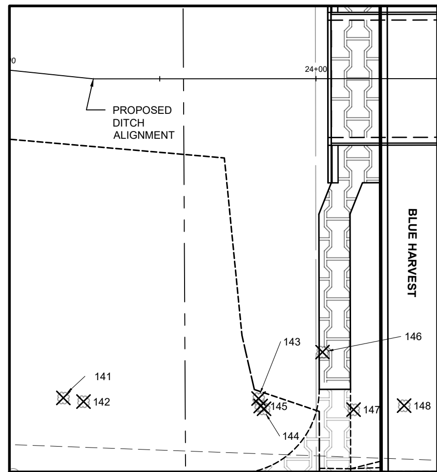
C 15 SOUTHEAST BLUE HARVEST SCALE: 1" = 30'
